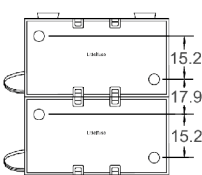
Gang Mount Setup
