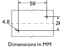
Mounting Diagram
