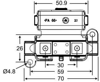
Mounting Diagram
